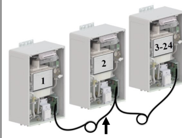
Cascade Cable
